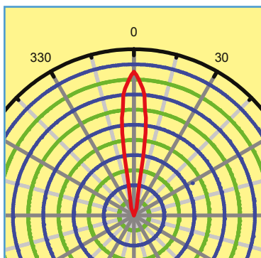
Polar Curve:
